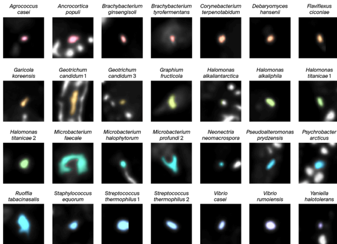
Figure 2. Example images of single cells of 28 of the predicted amplicon sequence variants that we detected by HiPR-FISH, with false coloring to highlight the cell of interest.
