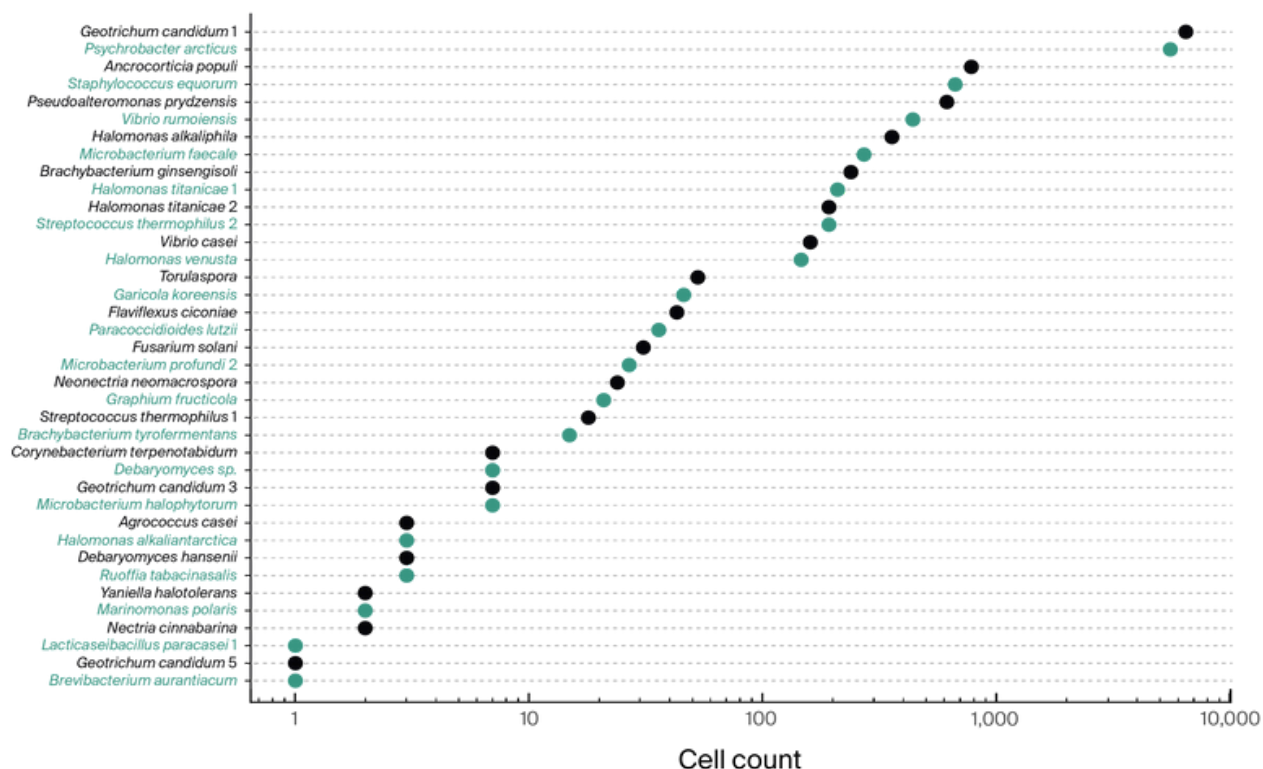
Figure 3. Log-transformed counts for each microbe detected across all FOVs for all cheeses.
