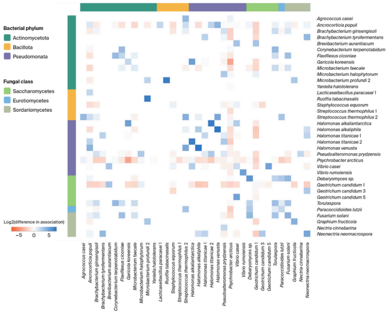
Figure 5. Spatial association heatmap showing the spatial enrichment of species relative to a randomly generated distribution across all rind FOVs.
