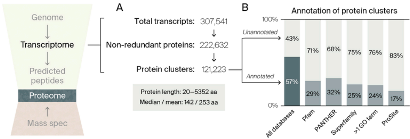
Figure 4. Processing and annotating protein clusters within our A. americanum transcriptome.
