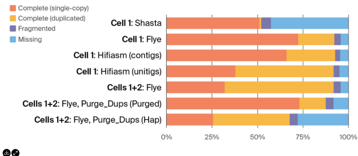
Figure 2. BUSCO results for each assembly.
