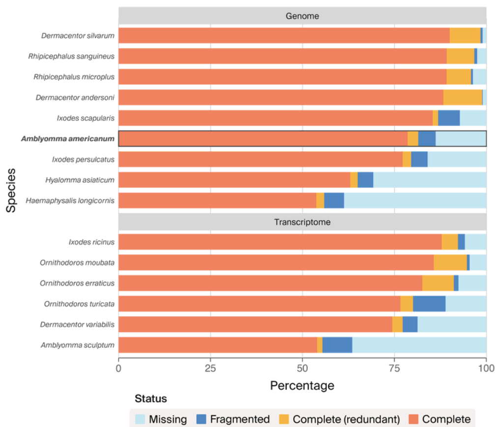
Figure 2. BUSCO scores for filtered tick proteomes compared to the filtered Amblyomma americanum proteome using the arachnida_odb10 lineage.
