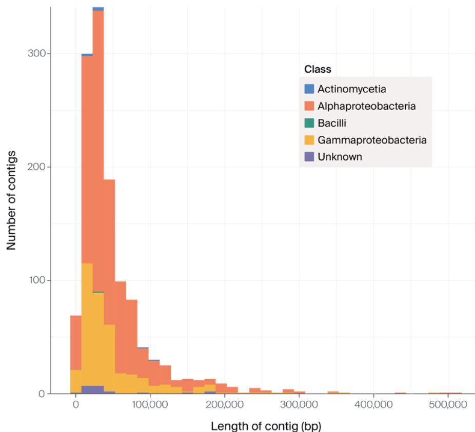
Figure 1. Contigs identified as bacterial or unknown and corresponding lengths.
