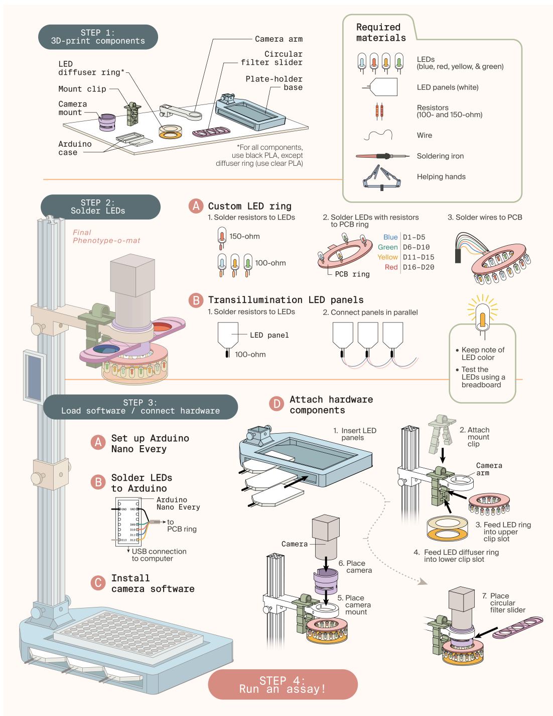
Figure 2. Assembling the phenotype-o-mat.
