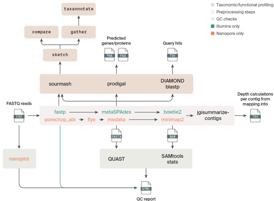
Figure 1. An overview of the steps in the metagenomics workflow.
