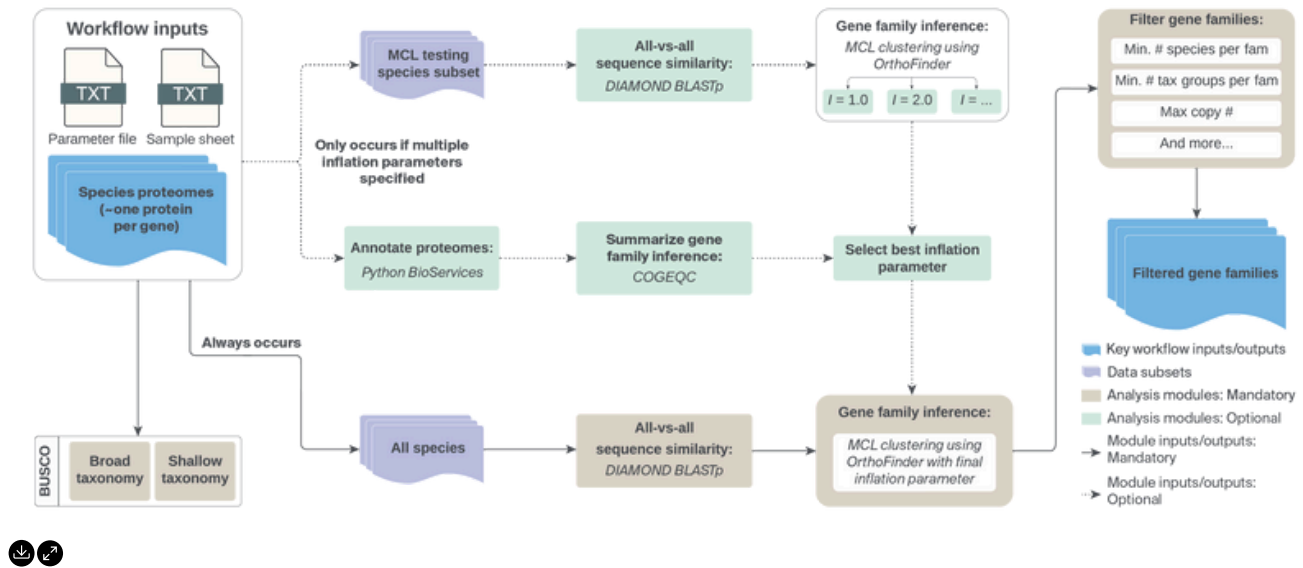
Figure 2. Detailed workflow diagram outlining the steps involved and methods implemented in the first stage of the workflow: gene family inference.
