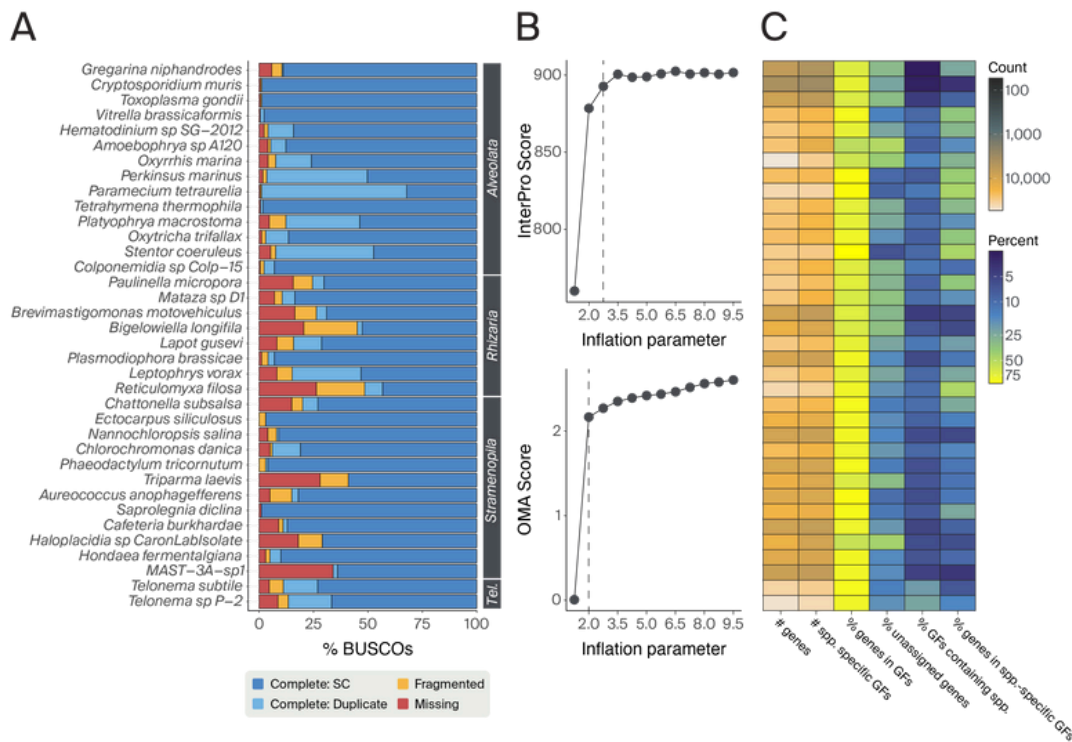
Figure 3. NovelTree produces BUSCO proteome quality summaries and high-level overview of results after gene family inference.
