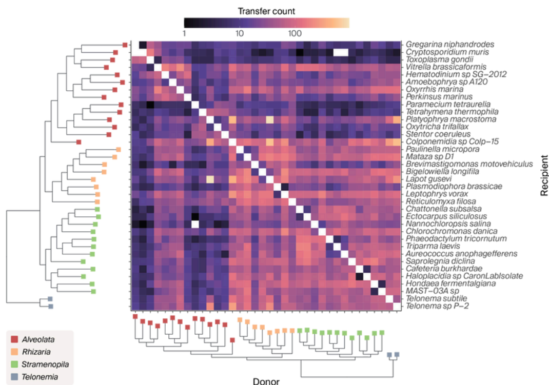
Figure 8. Heatmap depicting the number of horizontal transfer events among pairs of species, summed across all gene families as inferred under GeneRax's per-species model.
