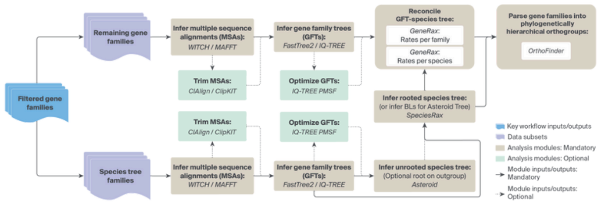
Figure 4. Detailed workflow diagram outlining the steps involved and methods implemented in the second stage of the workflow: phylogenetic inference, and inference of gene family evolution.
