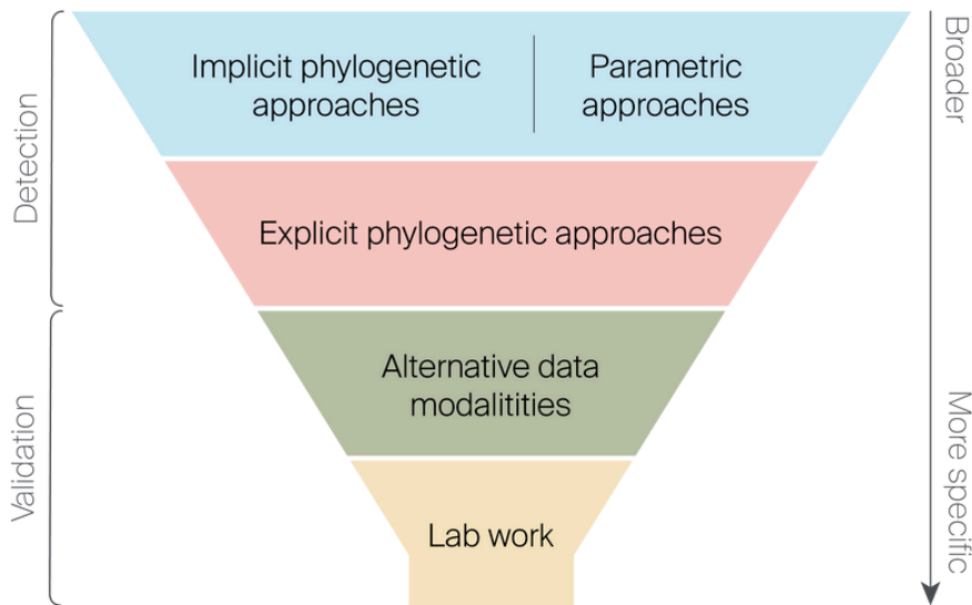
Figure 3. Funnel of methods for HGT screening and validation.
