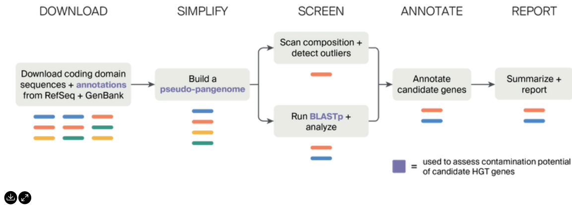
Figure 1. Conceptual overview of the HGT screening approach implemented in the preHGT pipeline.
