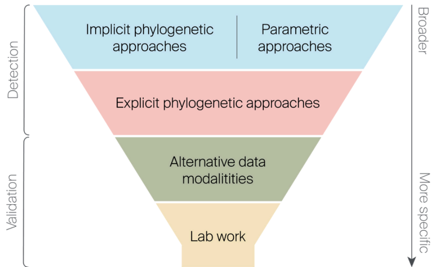
Figure 3. Funnel of methods for HGT screening and validation.
