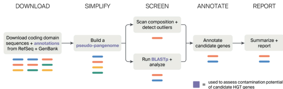
Figure 1. Conceptual overview of the HGT screening approach implemented in the preHGT pipeline.
