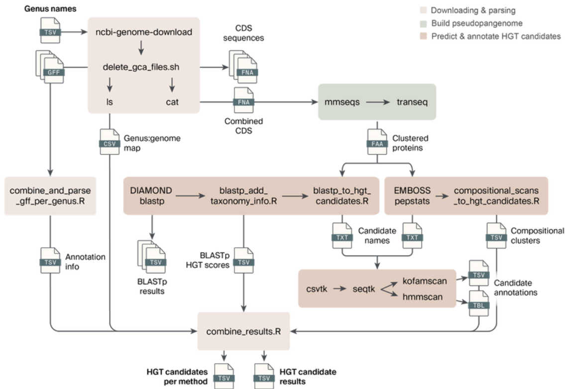
Figure 2. Overview of the preHGT pipeline steps, inputs, and outputs.
