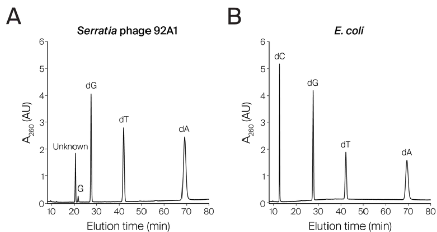
Figure 3. HPLC analysis reveals Serratia phage 92A1 uses an unknown nucleoside.
