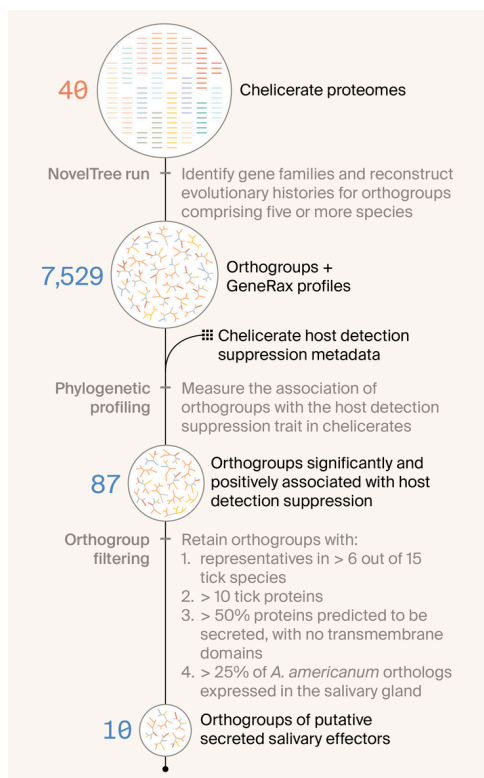
Figure 1. Our workflow for identifying gene families that help long-term feeders suppress host detection.
