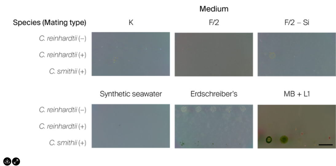
Figure 4. C. smithii can grow slowly on high-salt Erdschreiber's media and marine broth with L1 nutrients included.
