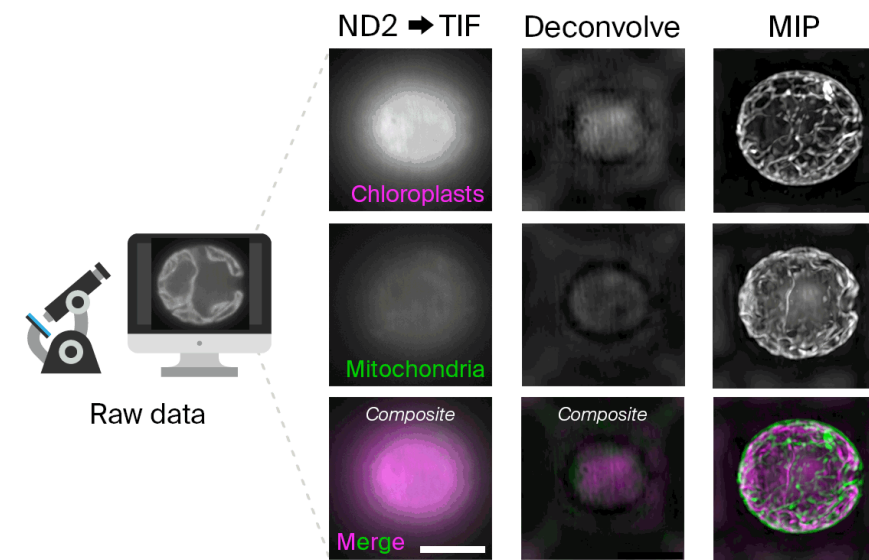
Figure 2. Overview of the image processing workflow to generate volumetric organelle data from Chlamydomonas parent species following high-resolution microscopy.
