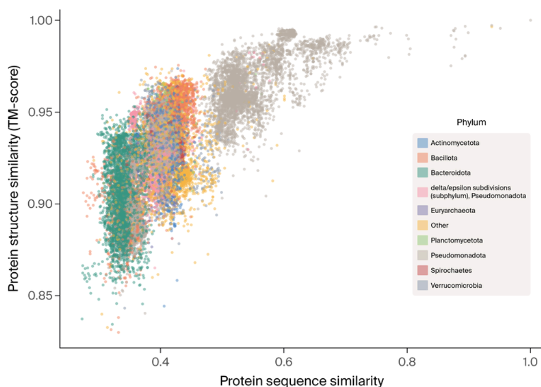
Figure 4. Pairwise all-v-all comparison of protein sequence and structural similarity (TM-score) to the Accumulibacter PPK1 reference protein.
