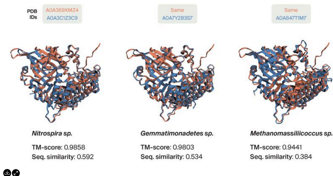
Figure 3. Structural comparisons of Accumulibacter PPK1 to PPK1 structures from other phyla that are significant in wastewater treatment processes.
